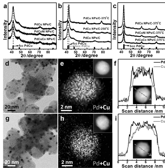
Figure 2. XRD patterns of a) PdCuM NPs/C, b) PdCu NPs/C at different heat treatment temperatures, and c) PdCuM NPs/C at 375°C heat treatment. Representative d,g) TEM image, e,h) HAADF-STEM-EELS elemental mapping and f,i) STEM-EELS line scans of single PdCu NPs/C without and with 375°C treatment.
